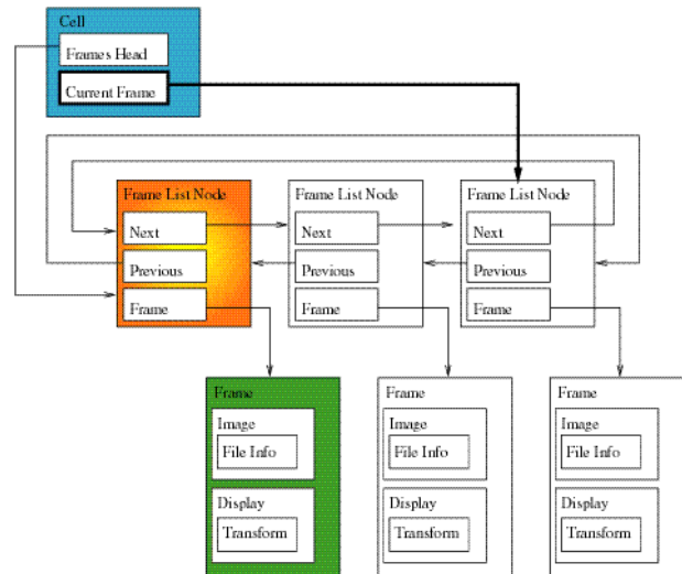
Figure 3 Organization of cell data includes a list of frames contained in the cell (circular doubly-linked list for framelist), pointer to current frame and each frame containing original and display data information.
