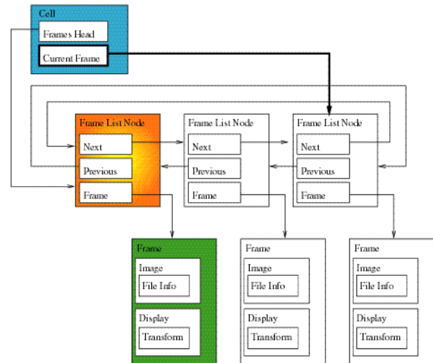
Figure 3 Organization of cell data includes a list of frames contained in the cell (circular doubly-linked list for framelist), pointer to current frame and each frame containing original and display data information.
